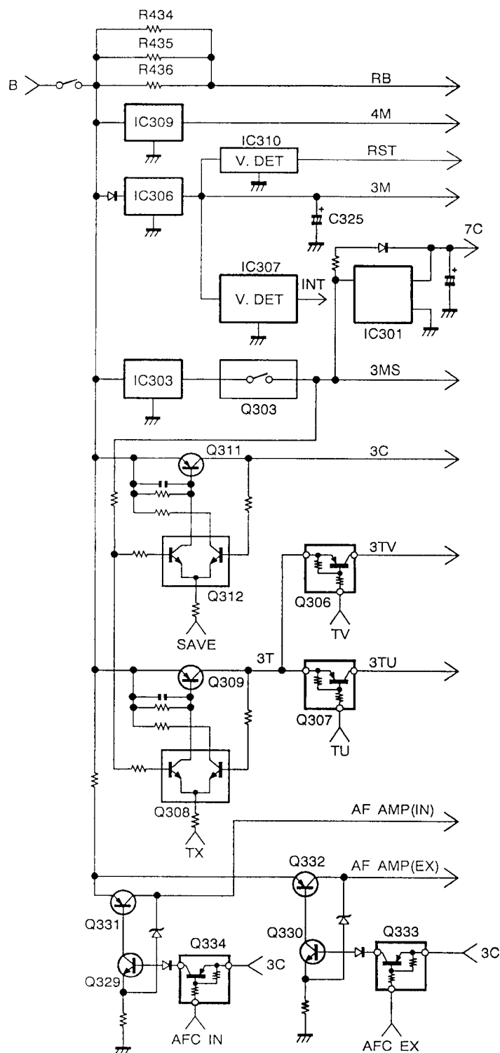
Fig. 8 Power supply circuit
