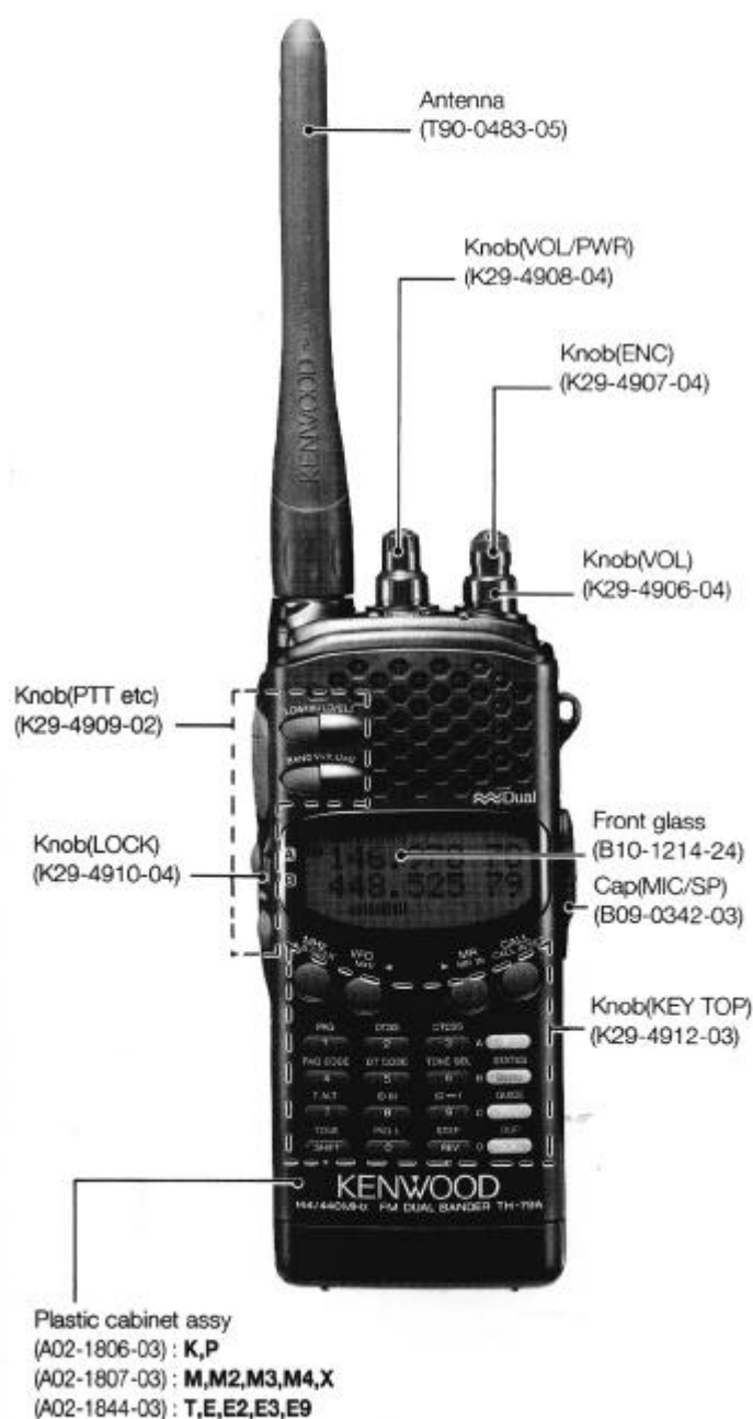
Photo is TH-79A.
