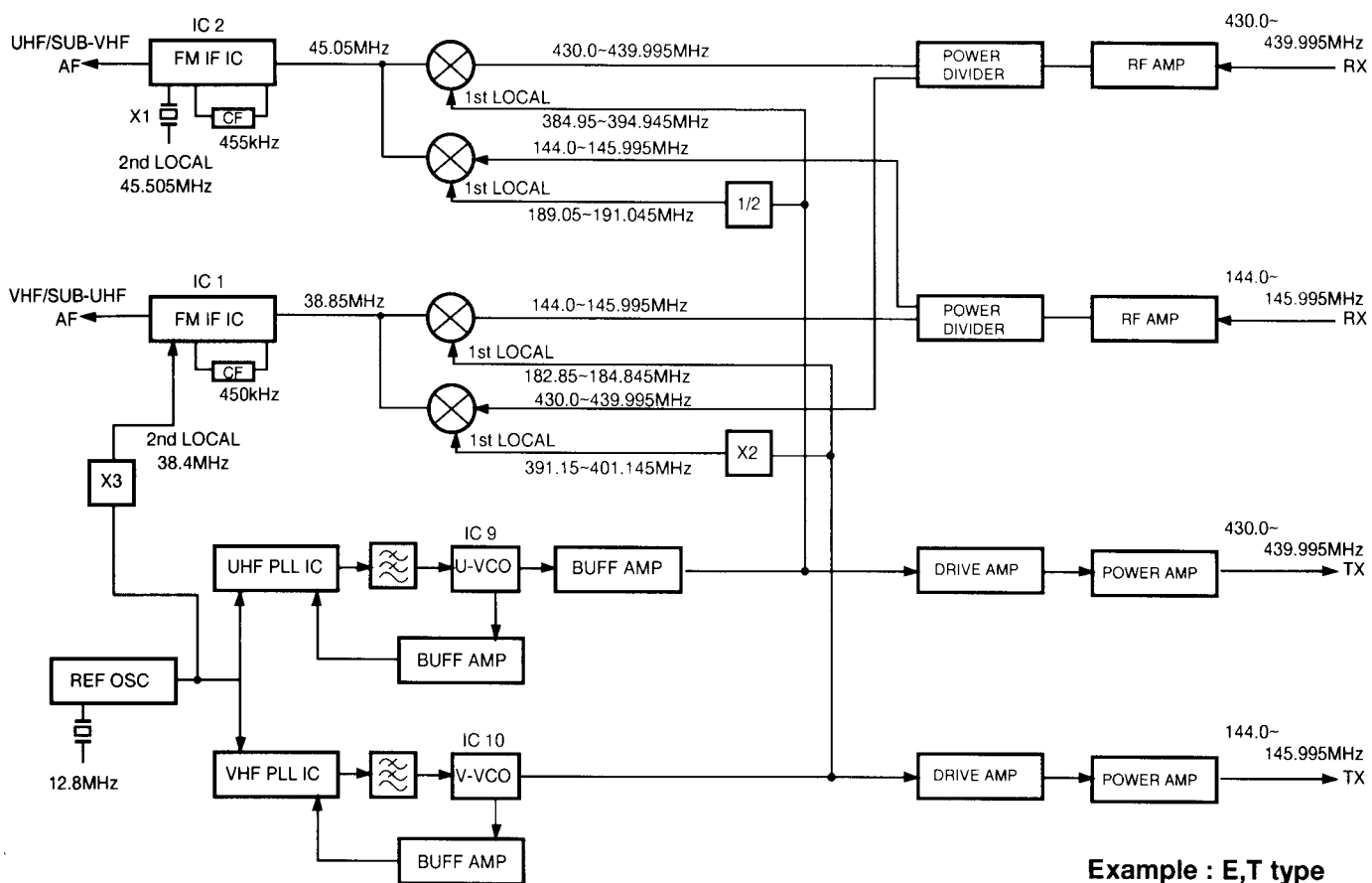
Fig.1 Frequency configuration
